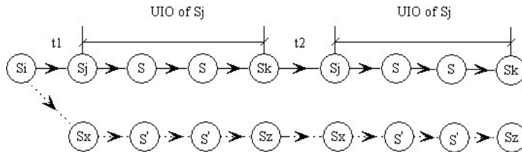
Figure 1: Fault Masked UIO Cycling
