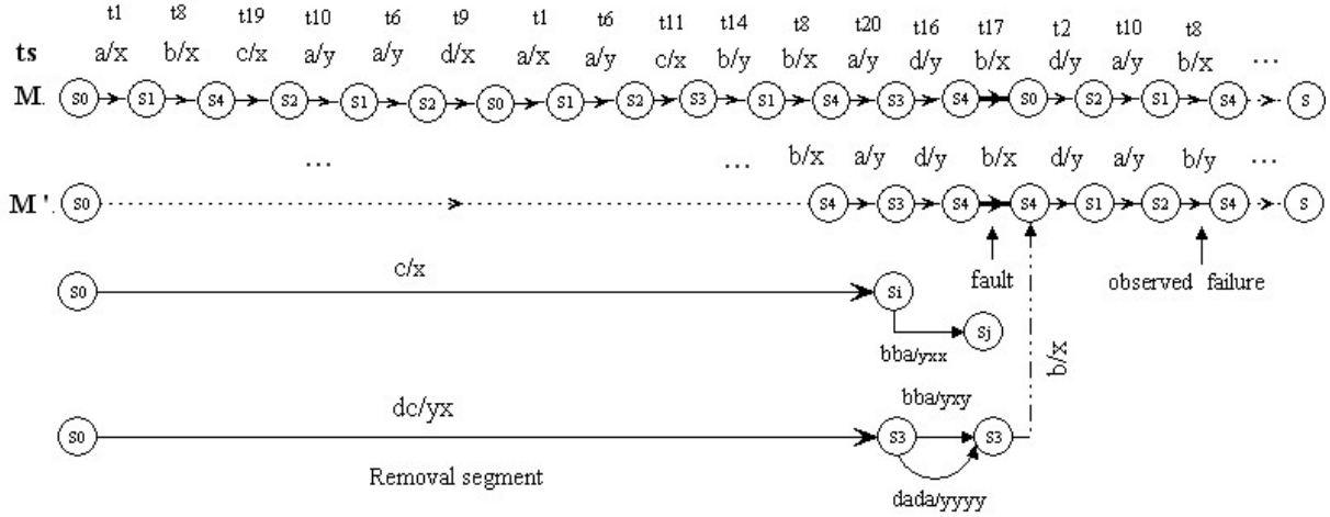
Figure 4: Fault detection and identification in M'
