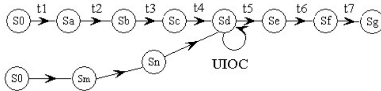
Figure 2: Reducing the size of a conflict set by applying a transfer sequence
