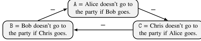
Figure 2. The epistemic graph has constraints \{p(B) > 0.5 \Rightarrow p(A) \leq 0.5, p(C) > 0.5 \Rightarrow p(B) \leq 0.5, p(A) > 0.5 \Rightarrow p(C) \leq 0.5\} . Given these constraints, we see that at most one argument can be believed.
