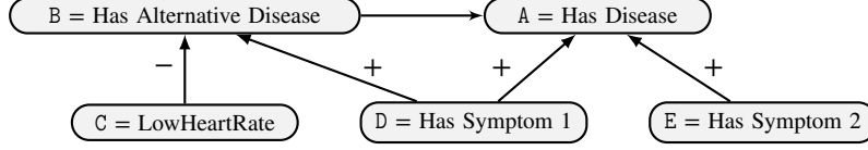
Figure 1. Example of an epistemic graph concerning diagnosis of a disease based on belief in symptoms and a differential diagnosis which in turn is based on a symptom and a test. The + (resp. -) label denote support (resp. attack) relations. Assume that if B is strongly believed, and D or E is strongly disbelieved, then A is strongly disbelieved, whereas if B is believed, and D or E is disbelieved, then A is disbelieved. Furthermore, if D and E are believed, then A is believed. These constraints could be reflected by the following formulae: \varphi_1 : p(B) > 0.8 \wedge p(D \vee E) < 0.2 \Rightarrow p(A) < 0.8 ; \varphi_2 : p(B) > 0.5 \wedge p(D \vee E) < 0.5 \Rightarrow p(A) < 0.5 ; \varphi_3 : p(D \wedge E) > 0.5 \Rightarrow p(A) > 0.5 ; \varphi_4 : p(C) > 0.5 \Rightarrow p(B) \leq 0.5 ; And \varphi_5 : p(C) \leq 0.5 \Rightarrow p(B) > 0.5 .
