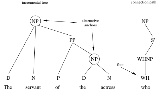
Figure 1. The two main syntactic interpretations of sentence (16) can be obtained by attaching the same CP to one of the two alternative anchors. In general, several CPs and several attachments for each CP are possible.
