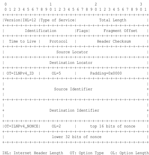
Figure 2: ILNPv4 packet header with optional Nonce
