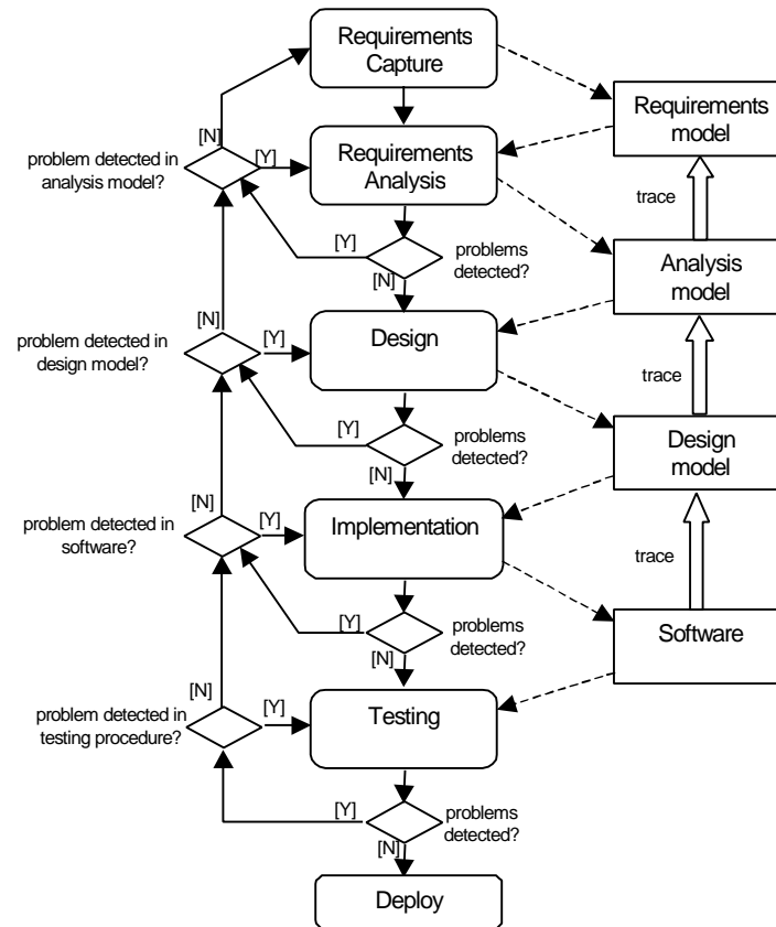
Figure 5: Model of Development Process Activities
