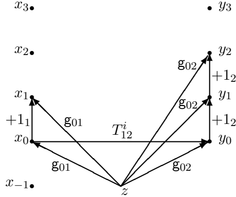
FIGURE 2. Representation implies Tiling
