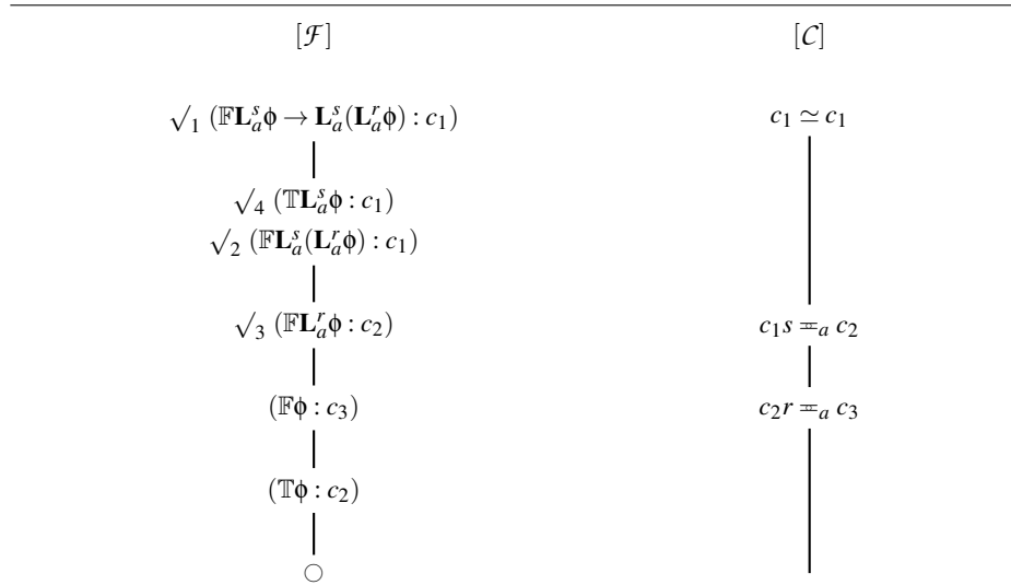
Figure 8. Tableau for \mathbf{L}_a^s \phi \rightarrow \mathbf{L}_a^r (\mathbf{L}_a^s \phi)
