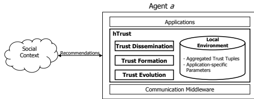
Fig. 1. hTrust Overview.
