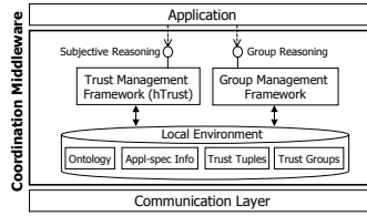
Fig. 5. Coordination Middleware.
